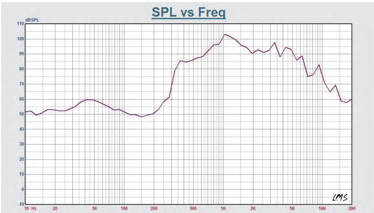
Frequency Response
